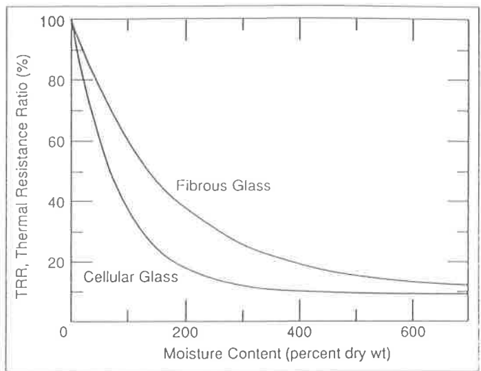
Figure 5 TRR vs. moisture content relationships for fibrous glass and cellular glass.
