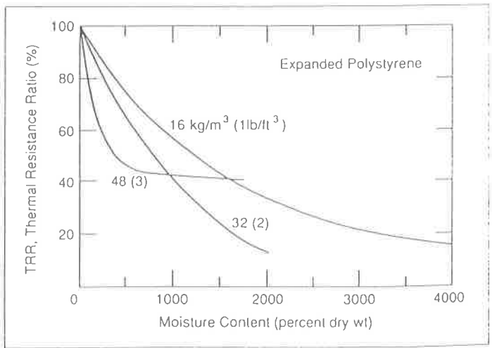
Figure 7 TRR vs. moisture content relationships for 16, 32 and 48 kg/m (1, 2 and 3 pcf) expanded polystyrene.
