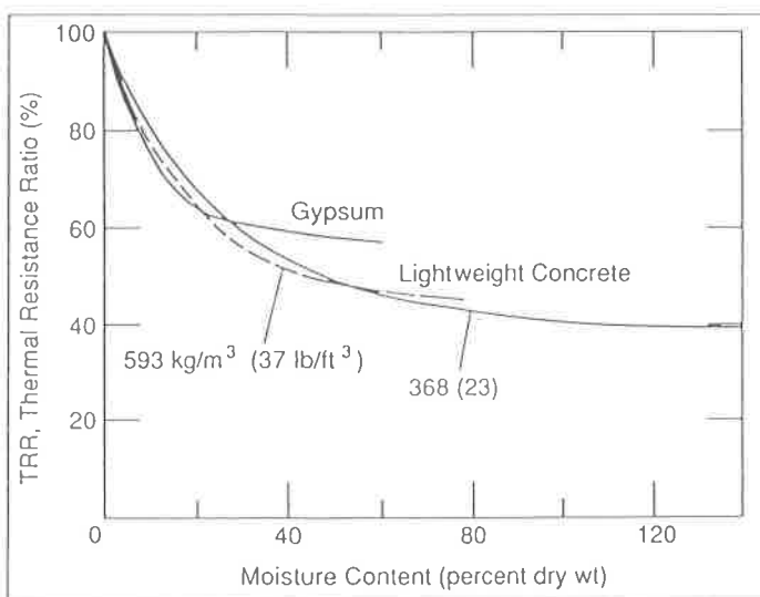
Figure 6 TRR vs. moisture content relationships for gypsum and 369 and 594 kg/m (23 and 37 pcf) lightweight concrete.
